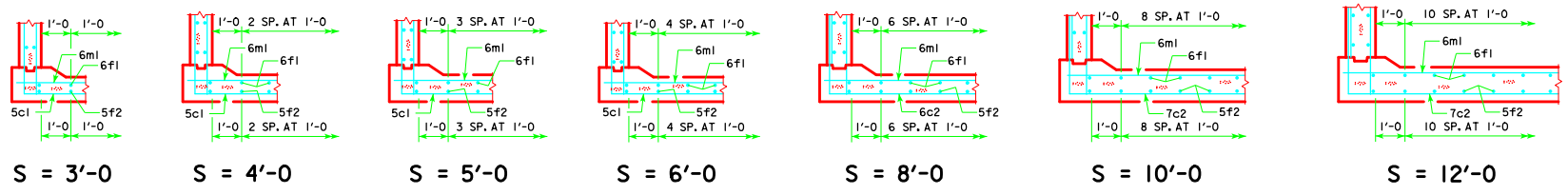
FLUME FLOOR HALF SECTIONS (NORMAL TO FLOWLINE)
