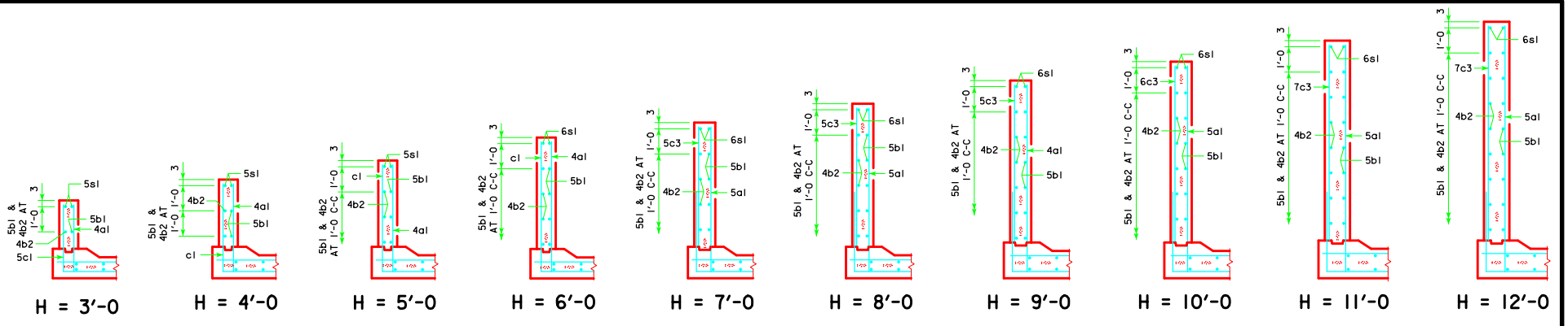
FLUME WALL SECTIONS (NORMAL TO FLOWLINE)
