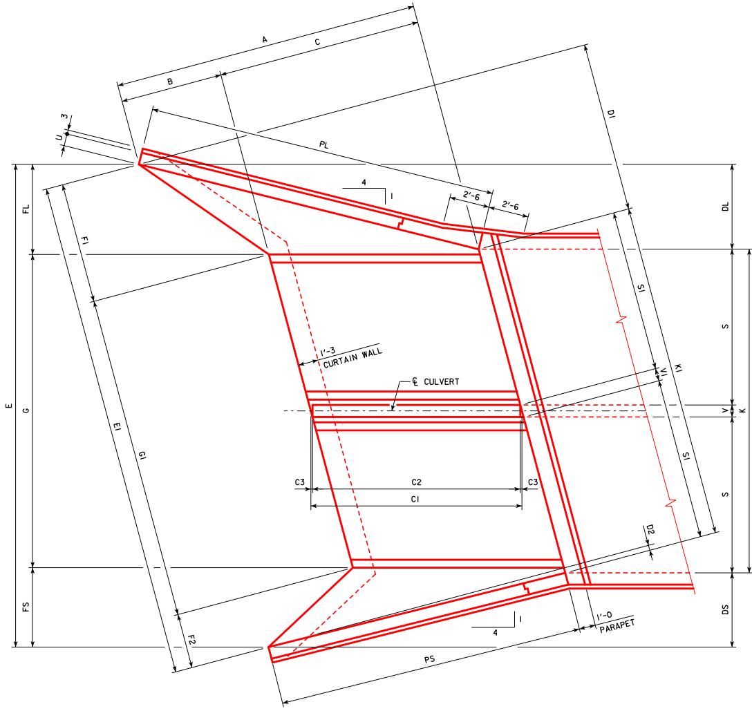
PLAN VIEW
